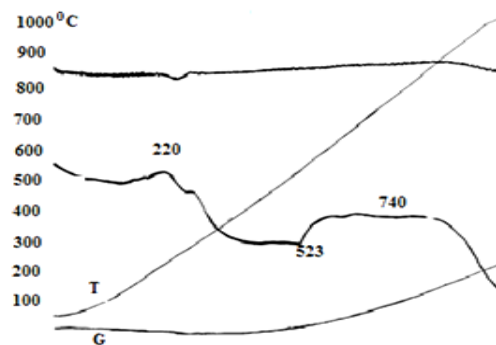
Fig. 2. DTA/TG curves of the Uvgundatsan iron ore.
